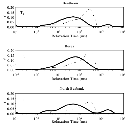
Fig. 15 T 1 relaxation time distributions of the sandstones after D 2 O brine diffusion (solid curve) compared to bulk SMY crude oil (dotted curve), scaled to oil saturation.
