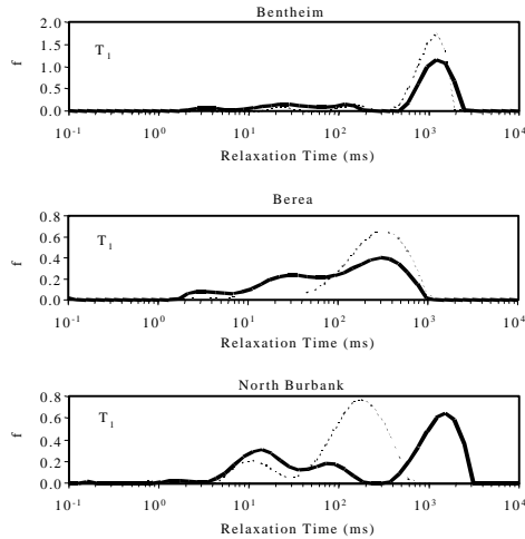
Fig. 14 T 1 relaxation time distributions of the sandstones after forced imbibition (solid curve) compared to 100% brine saturation (dotted curve).
