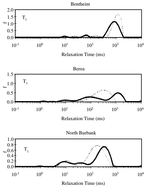
Fig. 7 T_1 relaxation time distributions of the sandstones after forced imbibition (solid curve) compared to 100% brine saturation (dotted curve).
