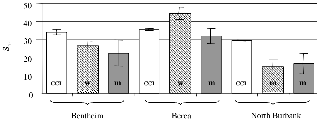
Fig. 17 Residual oil saturation from CCI (white bars), refined oil systems (hashed bars) and crude oil systems (shaded bars).
