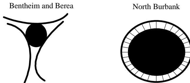
Fig. 11 Fluid distribution of crude oil systems after aging.
