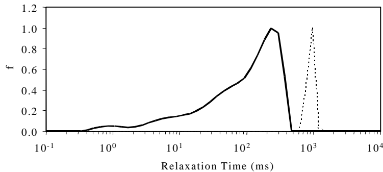
Fig. 3 Normalized T_2 distributions (echo spacing = 0.2 ms) of Soltrol (dotted curve) and SMY crude oil (solid curve).
