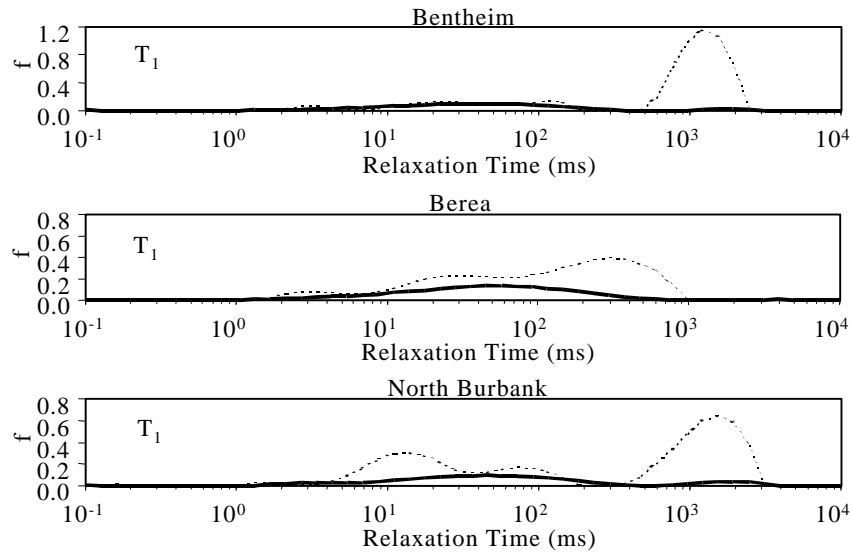
Fig. 13 T_1 relaxation time distributions of the sandstones after forced imbibition (dotted curve) and after D_2O brine diffusion (solid curve).
