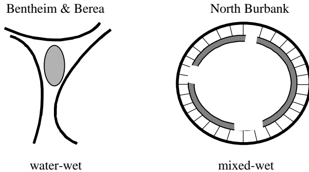
Fig. 9 Fluid distribution of refined oil systems after forced imbibition of brine.
