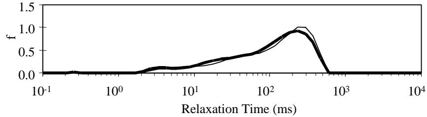
Fig. 12 T_1 relaxation time distributions of bulk SMY crude oil before aging (solid curve) and after aging (bold solid curve).
