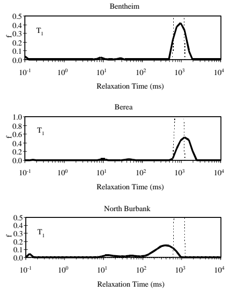
Fig. 8 T_1 relaxation time distributions of the sandstones after D_2O brine diffusion (solid curve) compared to bulk Soltrol (dotted curve).
