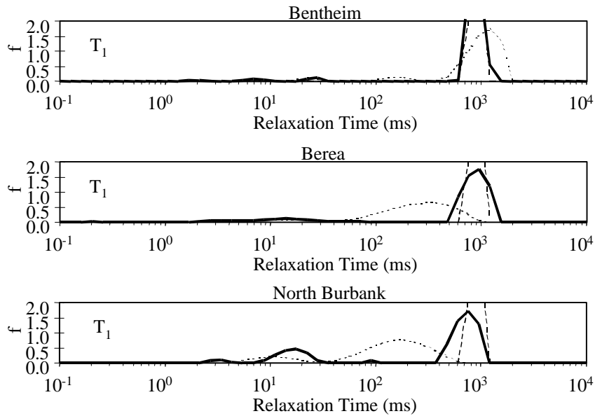
Fig. 4 T_1 relaxation time distributions of the sandstones at 100% brine saturation (dotted curve) and Soltrol saturated to S_{wir} (solid curve). The T_1 relaxation time distribution of bulk Soltrol is shown as the dashed curve.
