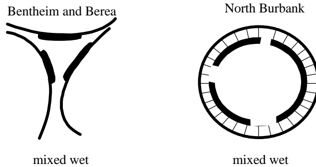
Fig. 16 Fluid distribution of crude oil systems after forced imbibition of brine.
