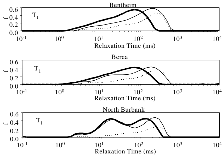
Fig. 10 T_1 relaxation time distributions of the sandstones with SMY crude oil saturated to S_{wir} before aging (solid curve) and after aging (bold solid curve). The T_1 relaxation time distribution of bulk SMY crude oil, scaled to oil saturation, is shown as the dotted curve.
