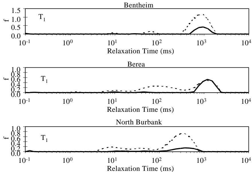
Fig. 6 T_1 relaxation time distributions of the sandstones after forced imbibition (dotted curve) and after D_2O brine diffusion (solid curve).
