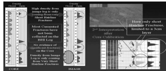
Figure 9 Comparison of original BHI and core interpretation, and revised BHI log after reviewing the BHI in the light of data from core.
