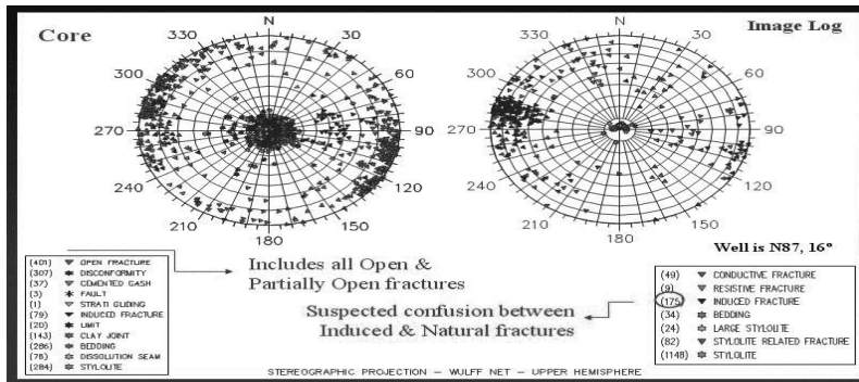
Figure 3 Core Stereonet Plot shows all open & partially open fractures. On BHI, 1148 Stylolites were not plotted to make the diagram clearer because those Stylolites features were confused with all other sedimentary and fracture features.
