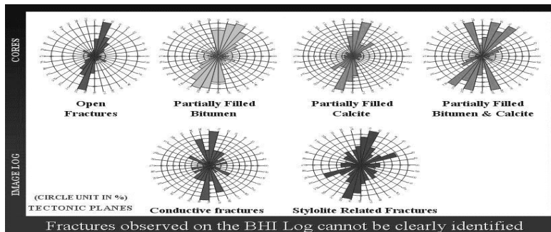
Figure 4 Core Strike Rose diagrams showing open fractures, partially open fractures and filling material. The BHI strike Rose diagrams showed only conductive and stylolite related fractures.
