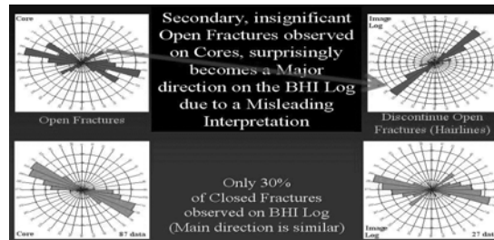
Figure 10 BHI interpretation could have lead to a wrongful view of fracture density and fractures direction of the different fracture families.
