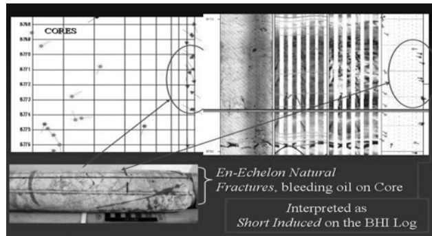
Figure 5 Many Natural ‘En Echelon’ fractures on cores reported as short induced fractures on BHI.
