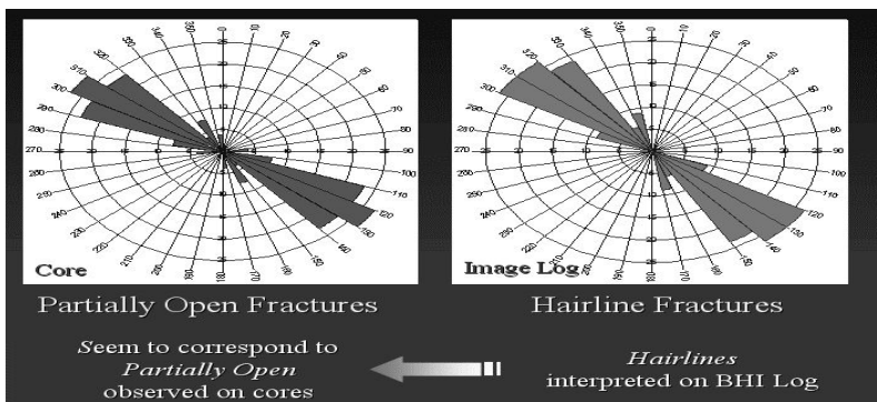
Figure 2 Partially Open Fractures Interpreted as Hairline Fractures on BHI log
