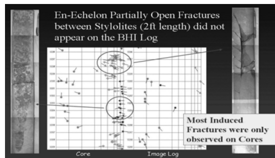
Figure 8 Photo on left side shows partially open fracture with Calcite (white) filling.
