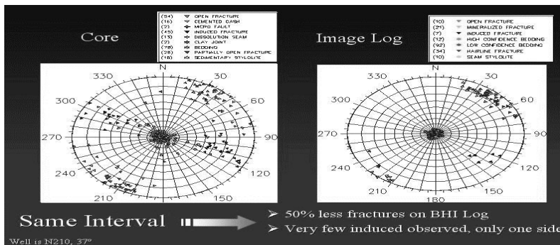
Figure 1 Stereonet Plot – Case #1
