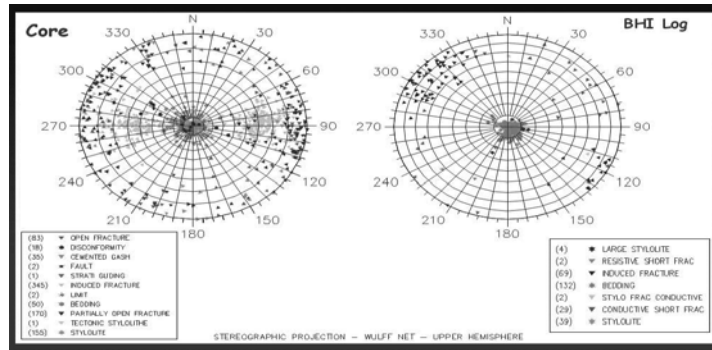
Figure 7 Stereonet plots – Core & BHI Log.
