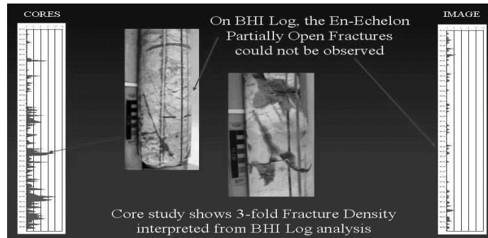
Figure 6 Many ‘En Echelon’ natural fractures did not appear on BHI log, leading to unrepresentative fracture density.
