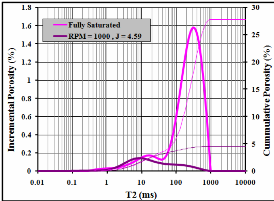
Figure 5 - Rock 98 T 2 cutoff measurement
