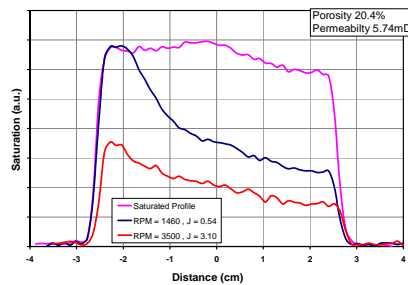
Figure 3 - MRI profiles of 1.5” diameter rock core plug during a air/Brine Pc measurement. The fully saturated profile is the relatively uniform profile showing the homogeneity of the rock. The remaining profiles are acquired after successively higher centrifuge speeds.
