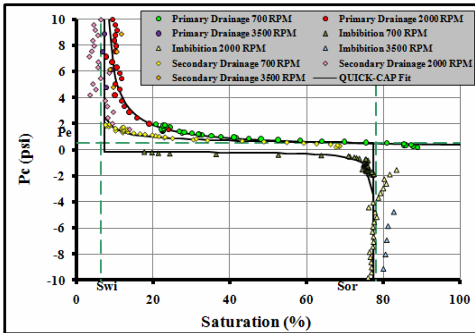
Figure 7 - Rock 42S oil/brine capillary pressure curves
