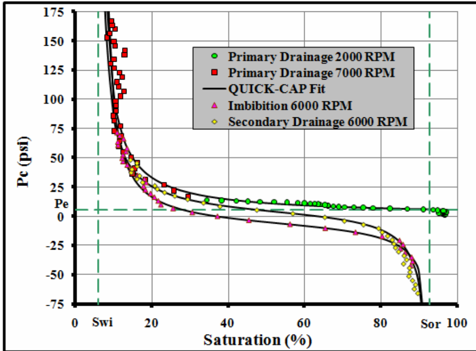
Figure 8 - Rock MT1 oil/brine capillary pressure curves
