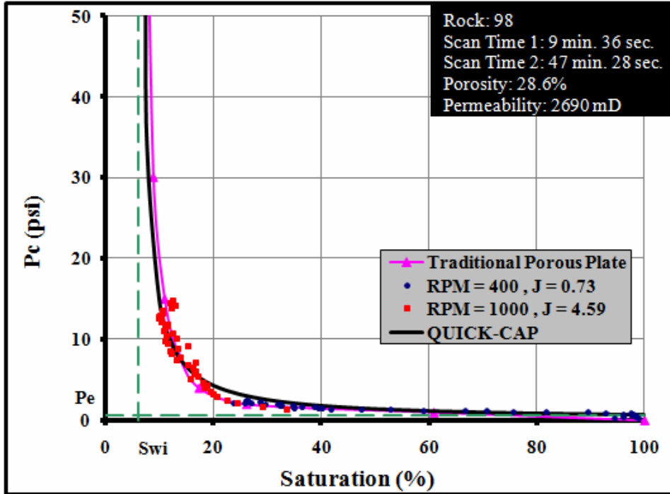
Figure 4 - Rock 98 Air/Brine Capillary pressure curve of a high permeability sandstone
