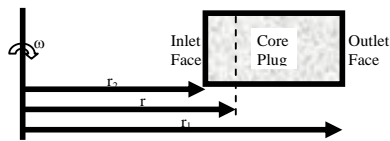
Figure 1 - Schematic of a rock core plug spinning in a centrifuge.
