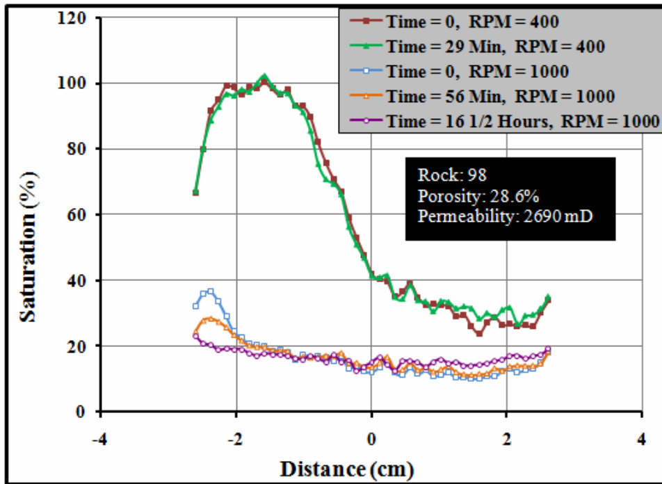
Figure 6 - Rock 98 redistribution of fluid following centrifugation
