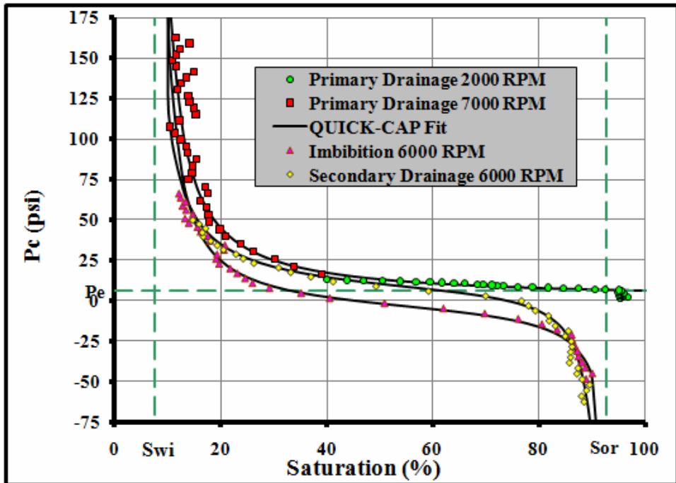
Figure 9 - Rock MT2 oil/brine capillary pressure curves
