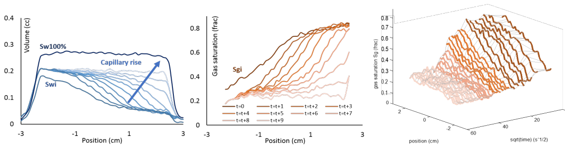
Figure 3: Capillary rise on Richmond sample prepared at 3000 rpm.
