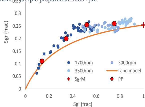
Figure 4: S_{gr} - S_{gi} results for the Richmond sample.
