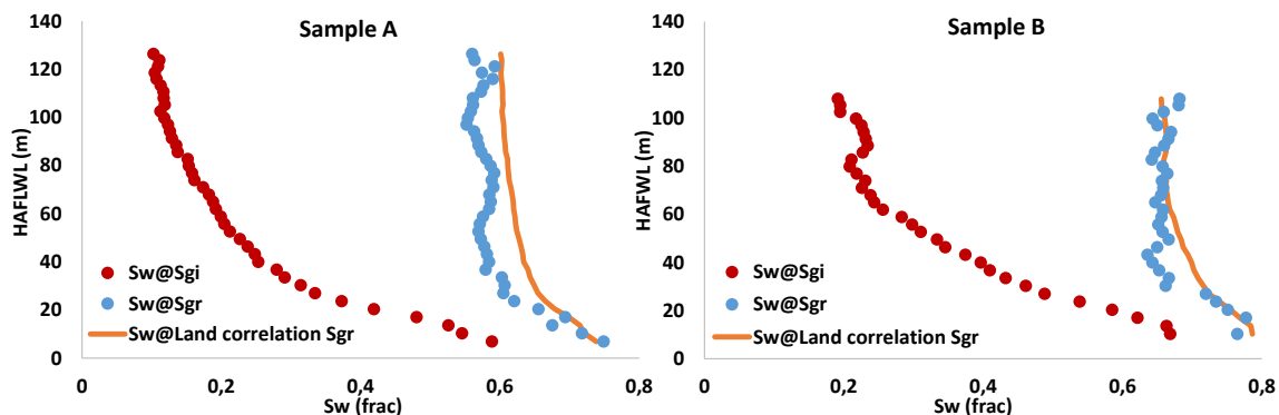
Figure 6: Results on reservoirs core plug represented as a function of height above free water level.
