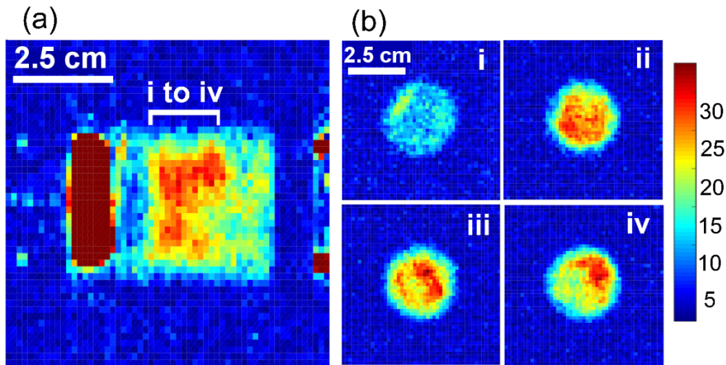
Figure 2. 2D slices from 3D \pi -EPI images of ^1\text{H} content in the methane hydrate system 26 hours after introducing methane gas. a) The strong methane reservoir signal is off scale at left in the image. No signal is apparent in the interface region of the sand pack. The water distribution is inhomogeneous reflecting a non-uniform distribution of hydrate in the sand pack. b) Four orthogonal slices from the data set of image (a) reveal the transverse inhomogeneity of hydrate formation. High image intensity is high water content and hence low hydrate conversion. The signal from the gas reservoir exceeds the dynamic range of the chosen display scale in Figure 2(a). Signal is simply mapped to the highest intensity of the chosen display range.
