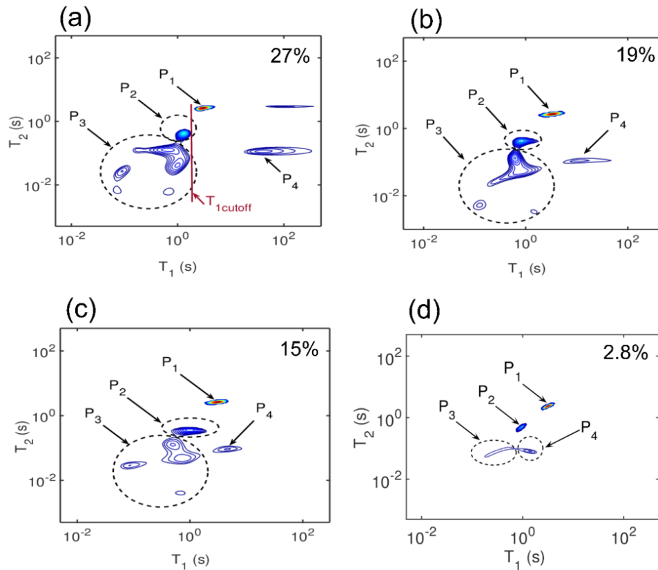
Figure 3. Bulk T_1 - T_2 measurement of the sand pack as a function of time after methane supply as hydrate forms. In each sub figure the residual water saturation in the pore space is at top right. (a) 4 hours (b) 14 hours, (c) 26 hours and (d) 212 hours. The peak labeled P_1 is bulk gas in the gas head, P_2 is bulk like water including water in threads of the apparatus, P_3 is residual water in the pore space. P_4 is assigned to residual gas in the pore space. T_{1cutoff} separates the gas phase peaks from those of water in the system. The P_4 peak shifts from long T_1 to shorter T_1 , as hydrate forms. Bulk T_1 - T_2 measurements, represented in Figure 3(a)-(d), have signal to noise ratios of 224, 154, 150 and 80. Variation in the regularization parameter did not change the major characteristics of the peaks [30].
