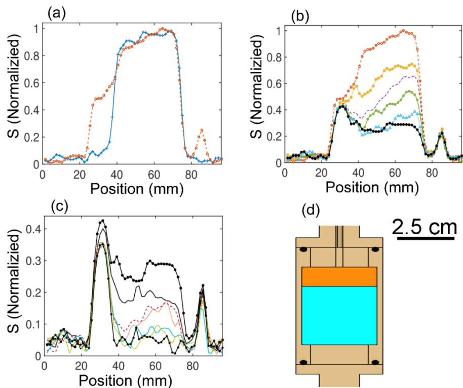
Figure 1. Space and time resolved ^1\text{H} fluid content profiles of hydrate formation. Methane penetrates the water saturated sand pack from a constant pressure gas head. Signal loss occurs when liquid water is converted to quasi solid hydrate. Hydrate forms first and most significantly near the gas head/sand pack interface. (a) profiles before and after introduction of the gas. The gas head is visible at left, 24 mm to 36 mm, while a small amount of water is visible at right displaced from the sand pack into threads of the sample vessel below the sand pack. Observed signal intensity is normalized by the maximum signal in the time zero profile. (b) ^1\text{H} fluid content profiles at 2, 2.25, 2.75, 3.45, 3.75 and 4 hours after introduction of the gas. (c) ^1\text{H} fluid content profile at 4, 14, 44, 68, 118, 152 and 217 hours after introduction of the gas. Hydrate formation has largely ceased approximately 120 hours after introduction of the gas but residual fluids, water and gas, remain in the pore space. Note the change in the y axis range in (c). (d) Schematic of
