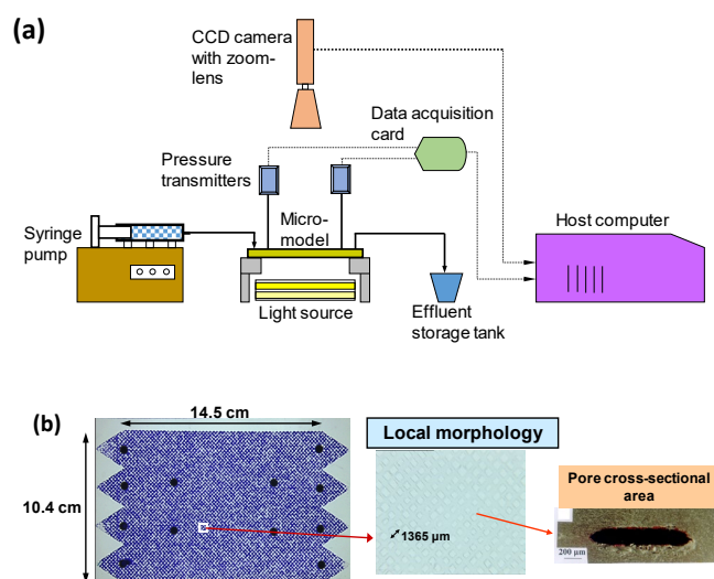
Fig. 2. (a) Schematic diagram of experimental setup. (b) Morphology of glass-etched pore network model.
