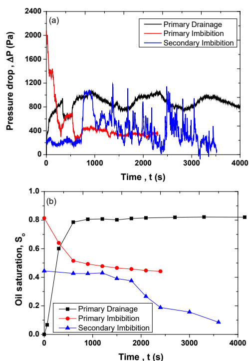
Fig.14. (a) Pressure drop, and (b) oil saturation, as a function of time. Pickering emulsion synthesized from IONP suspension with C_{Fe}=0.25 g/L and C_{NaCl}=0.25 M was injected at the secondary imbibition step.
