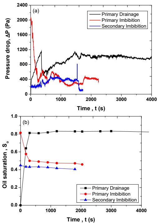
Fig.12. (a) Pressure drop, and (b) oil saturation, as a function of time. IONP suspension with C_{Fe}=0.5 g/L was injected at the secondary imbibition step.
