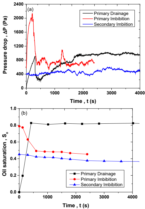
Fig.11. (a) Pressure drop, and (b) oil saturation, as a function of time. IONP suspension with C_{Fe}=0.25 g/L was injected at the secondary imbibition step.
