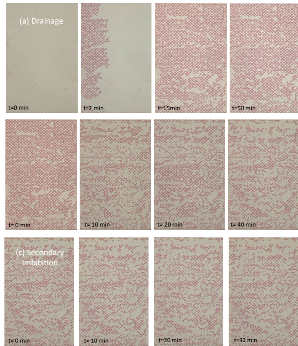
Fig.5. (a) Displacement of brine ( C_{NaCl}=0.25M ) by paraffin oil ( \mu=0.026 Pa s). (b) Displacement of paraffin oil by brine ( C_{NaCl}=0.25M ). (c) Displacement of residual paraffin oil by IONP suspension ( C_{Fe}=0.25 g/L).
